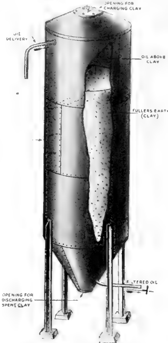
Fig. 3. Fuller's Earth Filter
